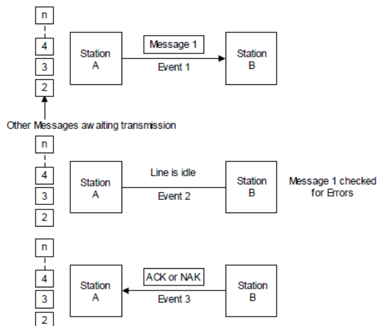
Gambar. 5: Stop and wait data link control
