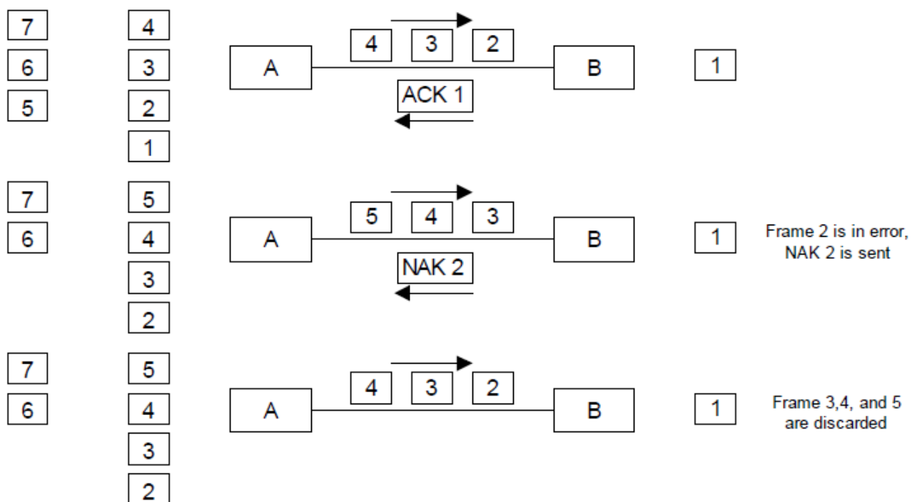
Gambar. 9: Go-back-N ARQ
